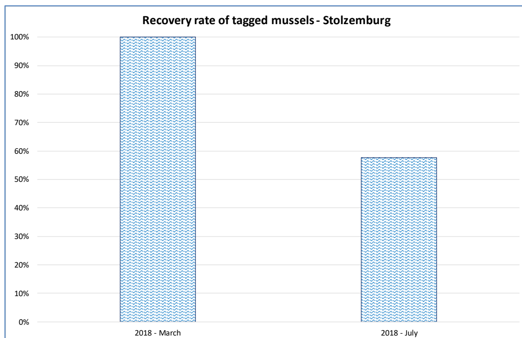
Figure 32: Recovery rate of tagged mussels at Stolzemburg
