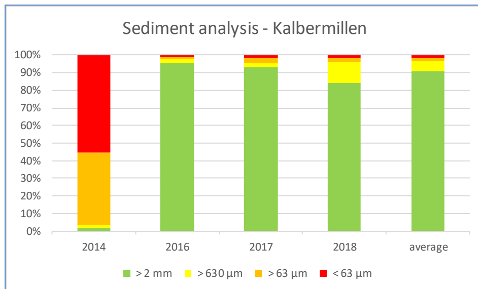
Figure 44: Sediment analysis of Kalbermillen mussels habitat
