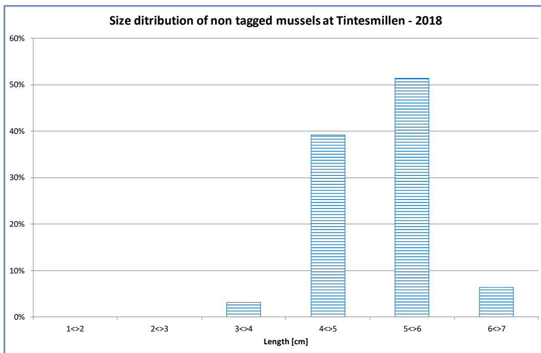
Figure 22: Size ditribution of non-tagged mussels at Tintesmilleren
