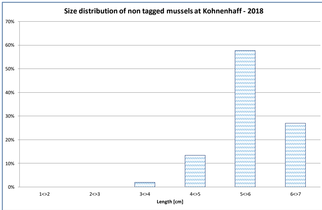
Figure 27: Size distribution of non-tagged mussels at Kohnenhaff
