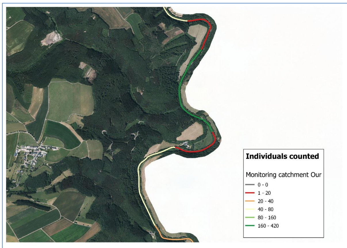
Figure 3: Mussel density at the Kalbermillen
