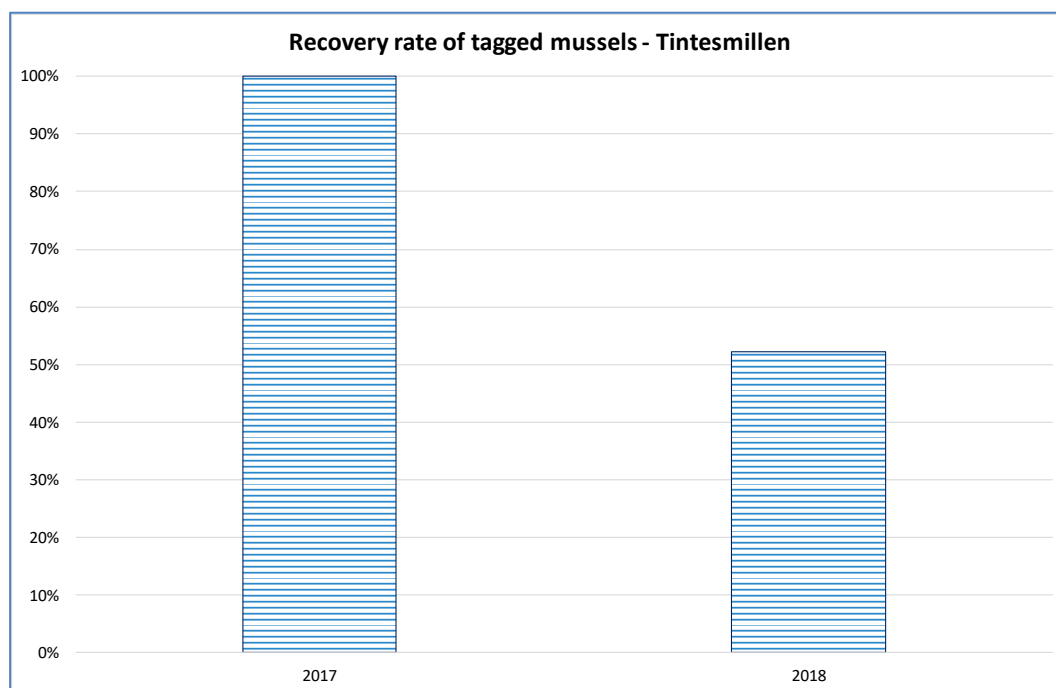
Figure 21: Recovery rate of tagged mussels at Tintesmilleren
