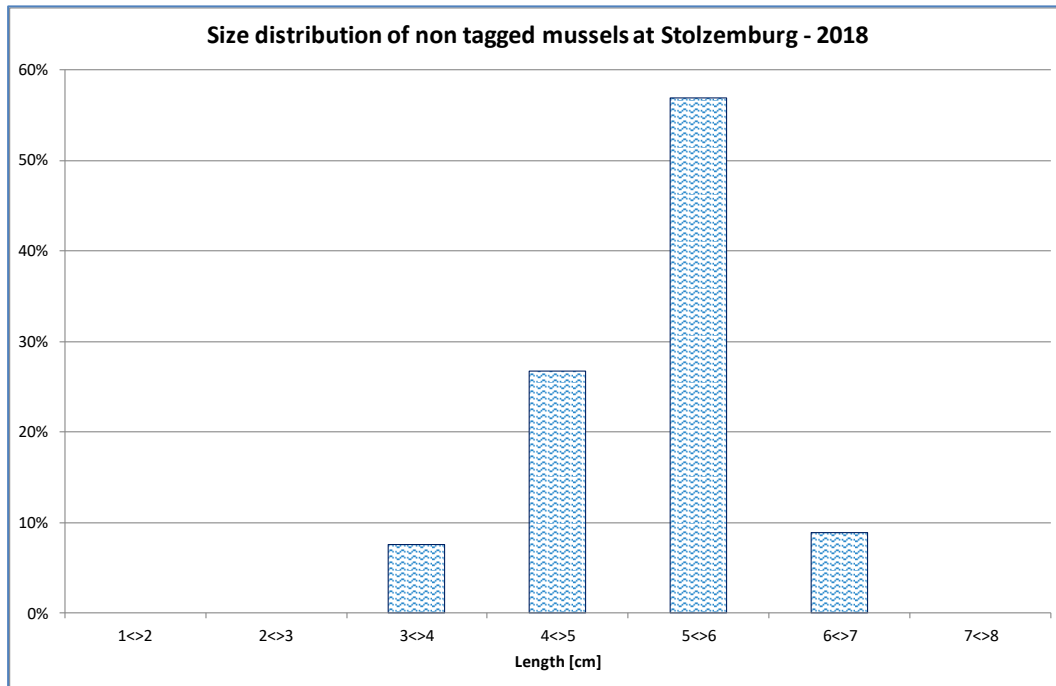
Figure 33: Size distribution of non-tagged mussels at Stolzemburg
