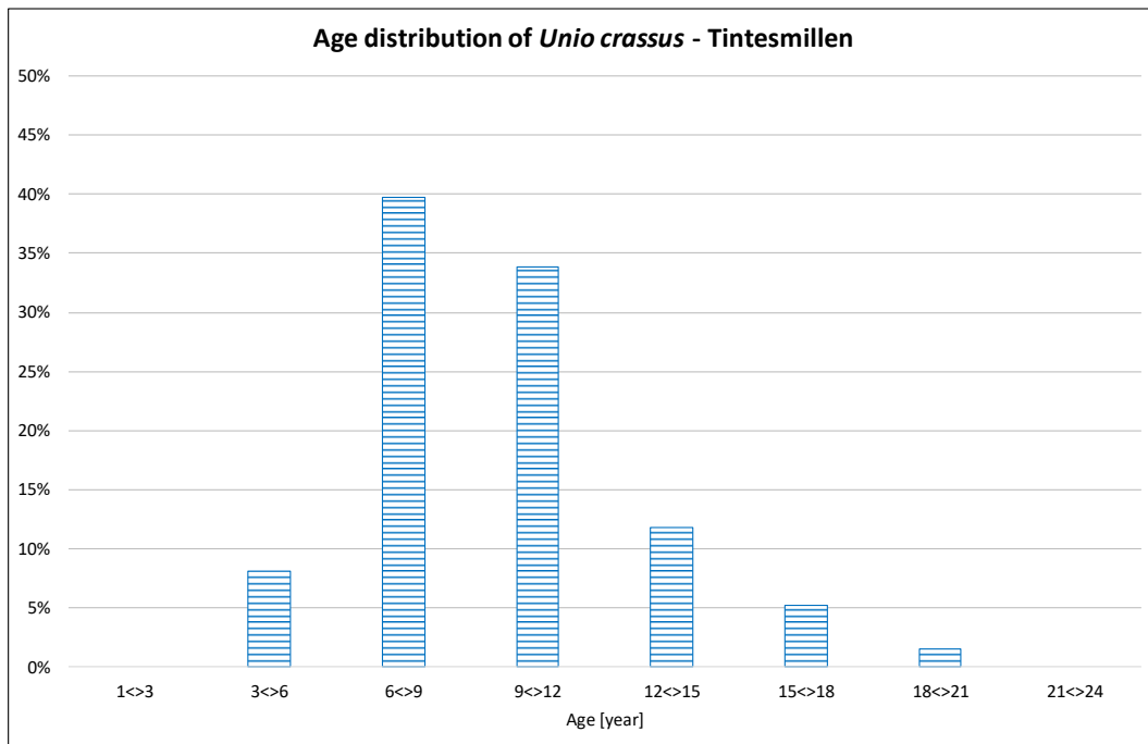
Figure 23: Age distribution of tagged mussels at Tintesmilen
