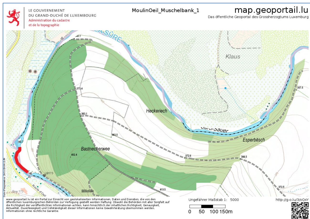
Figure 39: Tagged mussels at Moulin d'Oeil
