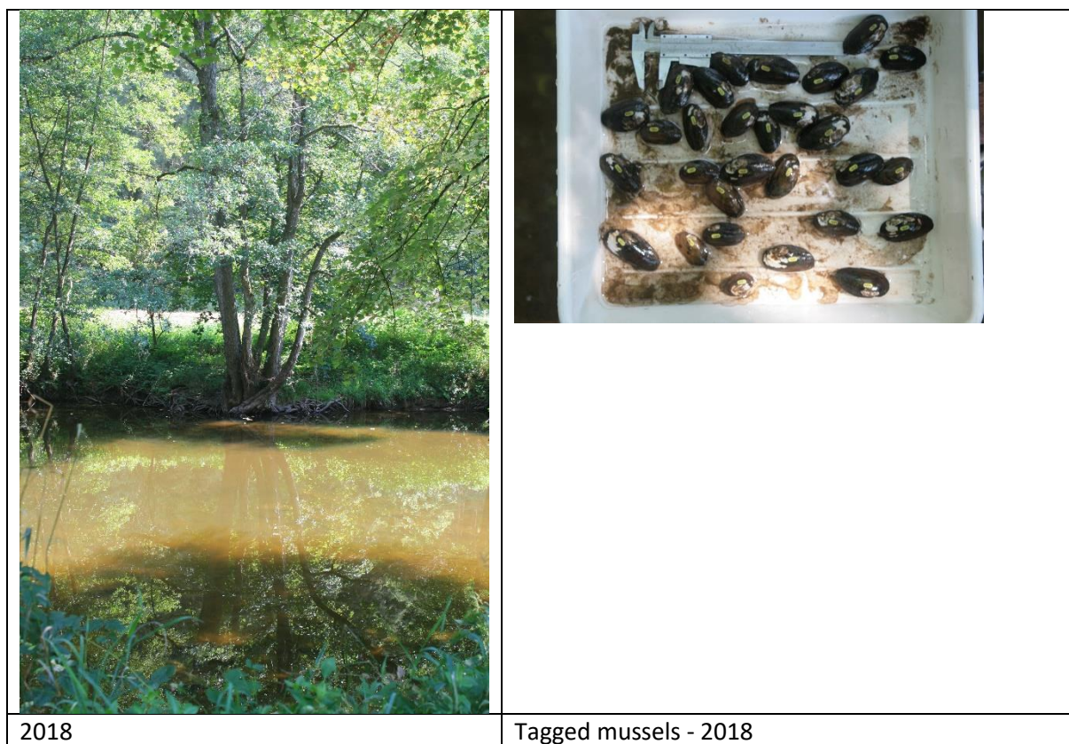
Figure 30: River Our at Stolzemburg
