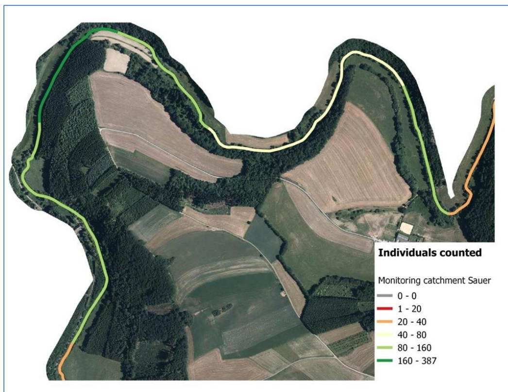
Figure 7: Mussel density at the Moulin d'Oeil
