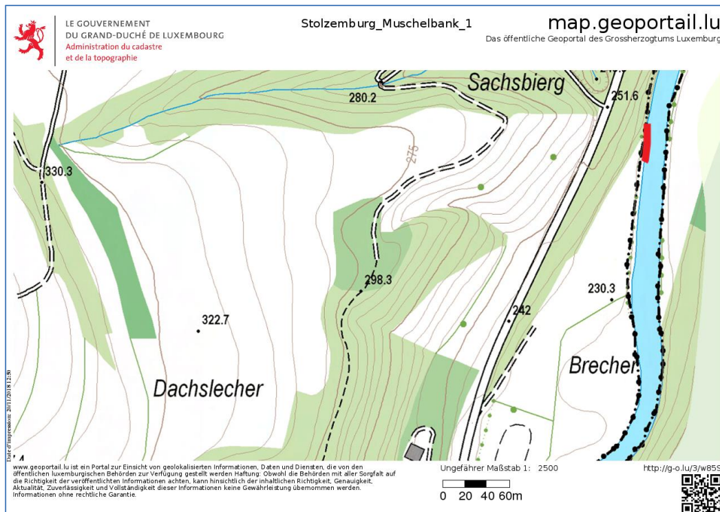
Figure 29: Tagged mussels at Stolzemburg
