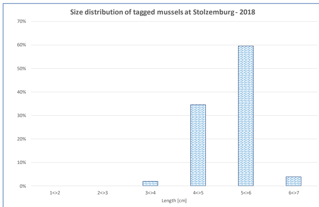
Figure 31: Size distribution of tagged mussels at Stolzemburg
