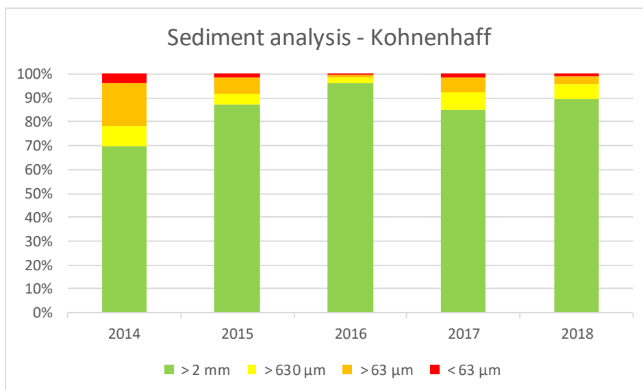
Figure 46: Sediment analysis of Kohnenhaff mussels habitat
