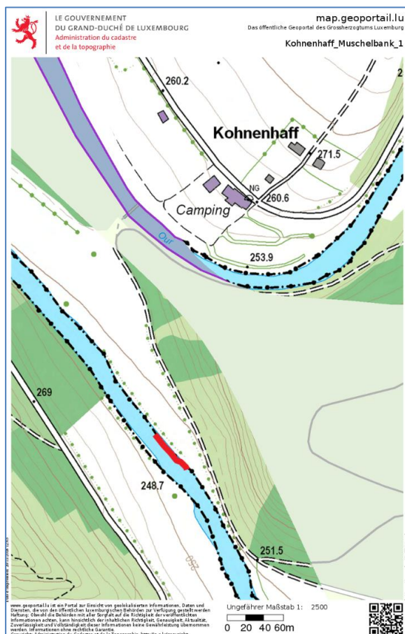
Figure 24: Tagged mussels at Kohnenhaff
