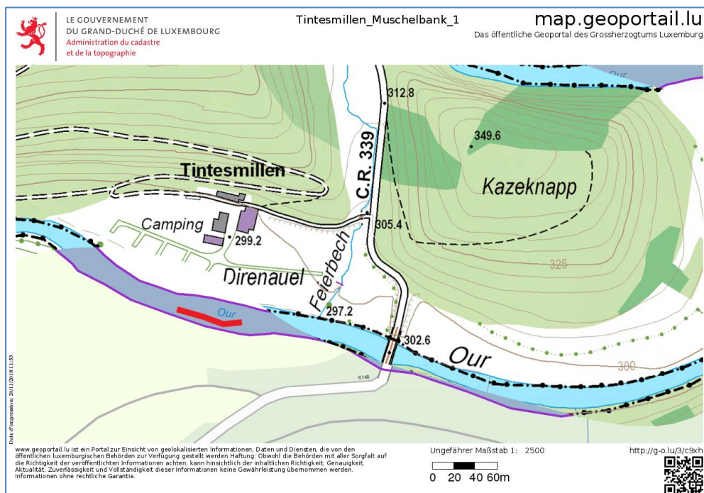
Figure 18: Tagged mussels at Tintesmiller
