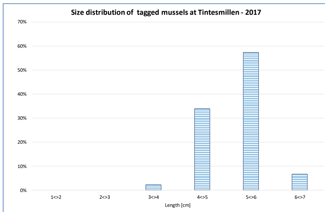
Figure 20: Size distribution of tagged mussels at Tintesmilleren
